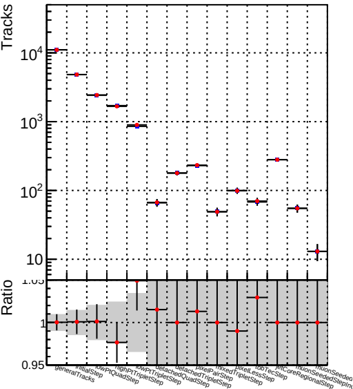
DQM_V0001_R000000001_Global_mkFiti100_RECO
