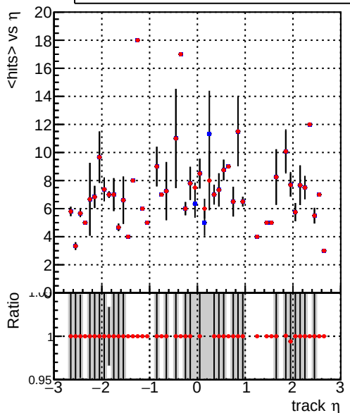
mean hits — DQM_V0001_R000000001_Global_mkFit100_RECO — DQM_V0001_R000000001_Global_mkFitALLCHAI100_RECO
