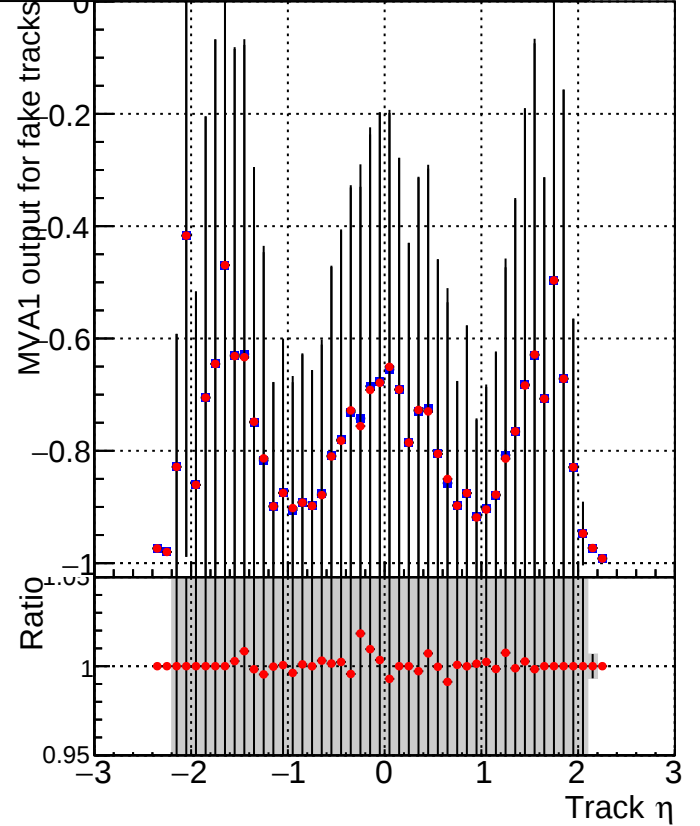
MVA1 of associated tracks (recoToSim) vs. track \eta Legend: ■ DQM_V0001_R000000001_Global_mkFiti100_RECO ● DQM_V0001_R000000001_Global_mkFitALLCHAi100_RECO
