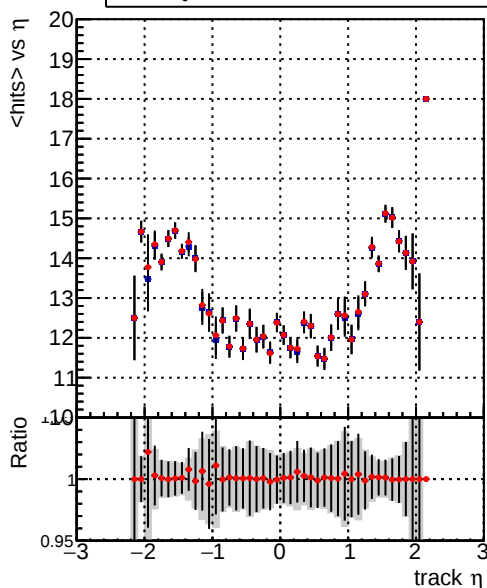
— DQM_V0001_R000000001_Global_mkFit100_RECO — DQM_V0001_R000000001_Global_mkFitALLCHAI100_RECO
