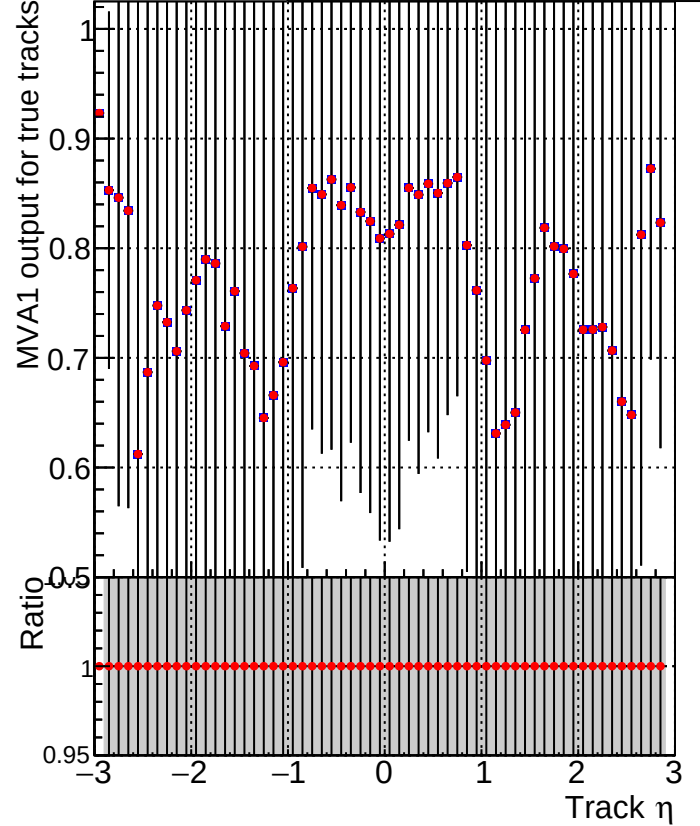
MVA1 of associated tracks (recoToSim) vs. track \eta Legend: ■ DQM_V0001_R000000001_Global_mkFit100_RECO ● DQM_V0001_R000000001_Global_mkFitALLCHAI100_RECO
