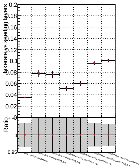
Fake rate vs. Legend Global mkFit100 RECO Blue line with dots DQM_V0001_R0000000001 Global mkFit100 Red line with dots DQM_V0001_R0000000001 Global mkFitALLCHAI100
