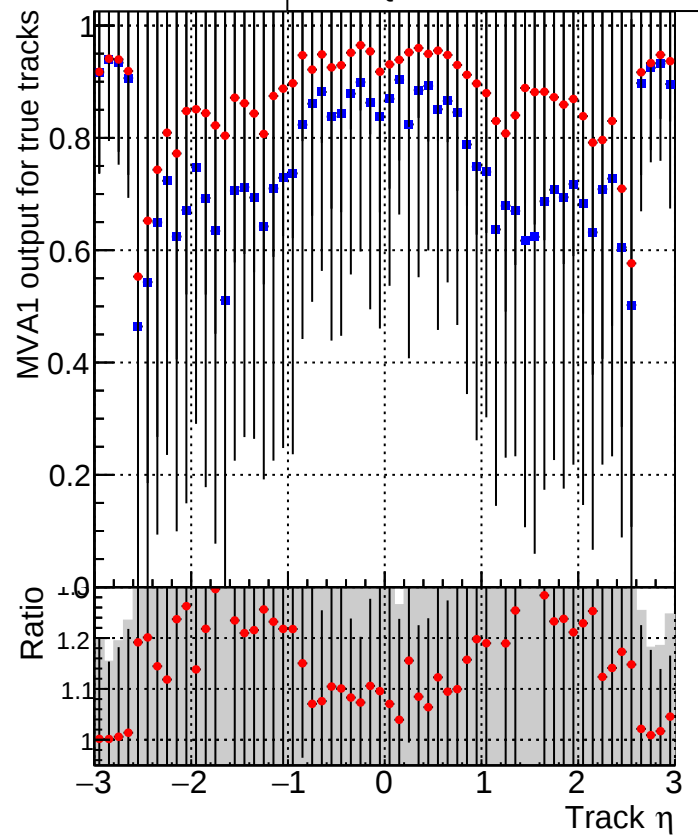
MVA1 of associated tracks (recoToSim) vs. track \eta Legend: Blue square: DQM_V0001_R000000001_Global_mkFiti100_RECO Red diamond: DQM_V0001_R000000001_Global_mkFitALLCHAi100_RECO
