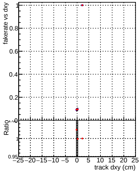
—●— DQM_V0001_R0000000001_Global_mkFit100_RECO —●— DQM_V0001_R0000000001_Global_mkFitALLCHAI100_RECO
