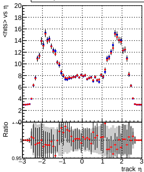
— DQM_V0001_R000000001_Global_mkFit100_RECO — DQM_V0001_R000000001_Global_mkFitALLCHAI100_RECO
