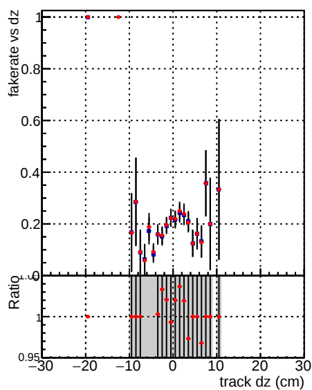
Fake rate vs dz —●— DQM_V0001_R0000000001_Global_mkFit100_RECO —●— DQM_V0001_R0000000001_Global_mkFitALLCHAI100_RECO
