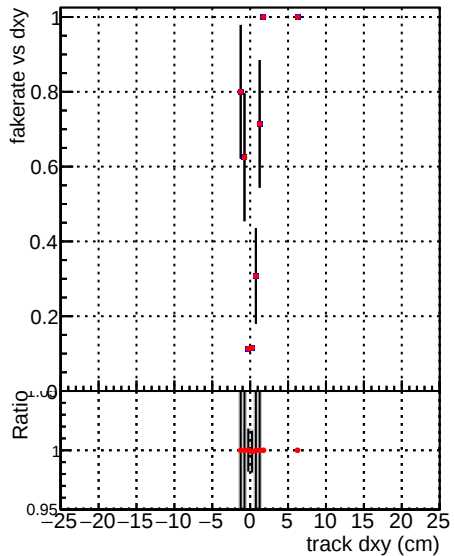
—●— DQM_V0001_R0000000001_Global_mkFit100_RECO —●— DQM_V0001_R0000000001_Global_mkFitALLCHAI100_RECO
