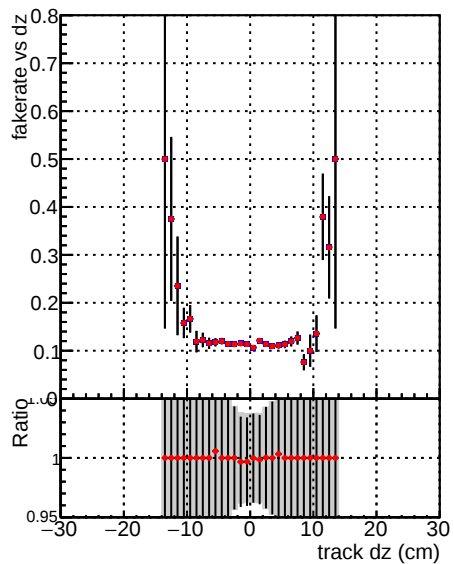
—●— DQM_V0001_R0000000001_Global_mkFit100_RECO —●— DQM_V0001_R0000000001_Global_mkFitALLCHAI100_RECO
