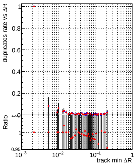
—●— DQM_V0001_R000000001_Global_mkFit100_RECO —●— DQM_V0001_R000000001_Global_mkFitALLCHAI100_RECO
