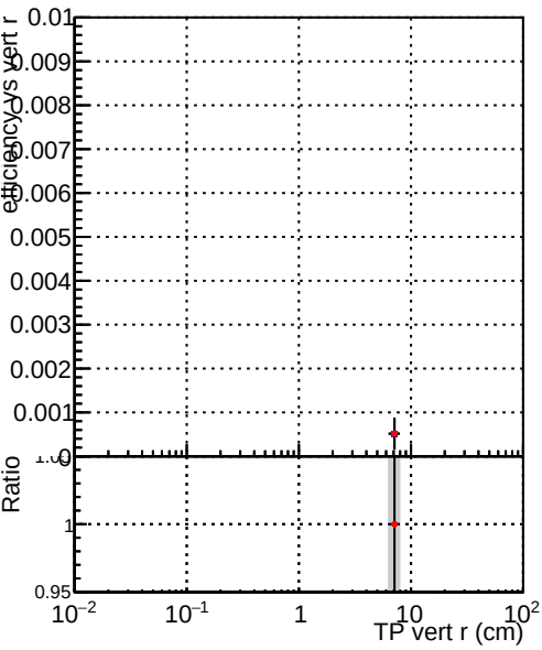
Efficiency vs vertpos Legend: DQM_V0001_R0000000001_Global_mkFit1000i0_RECO DQM_V0001_R0000000001_Global_mkFit1000mod_RECO
