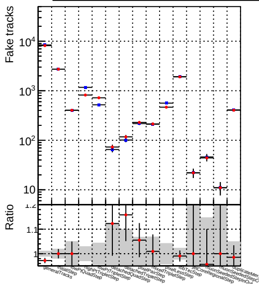
Number DOM V0001 R0000000001 Global mkFit1000mod RECO
