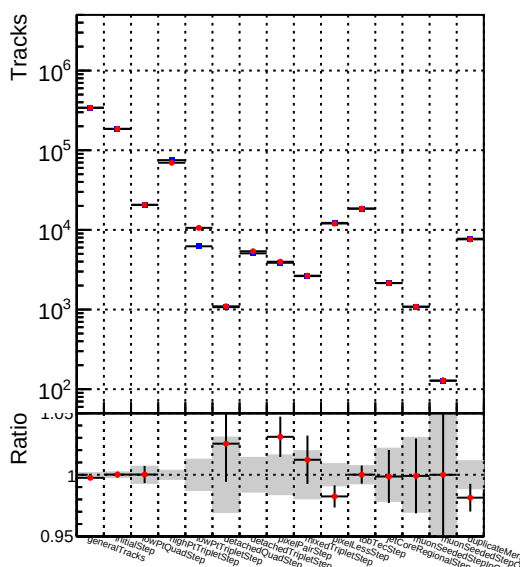
DOM V0001 R0000000001 Global mkFiti100i0 RECO
