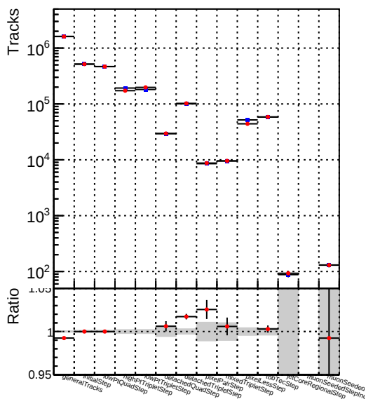
DQM_V0001_R000000001__Global__mkFiti100i0__RECO
