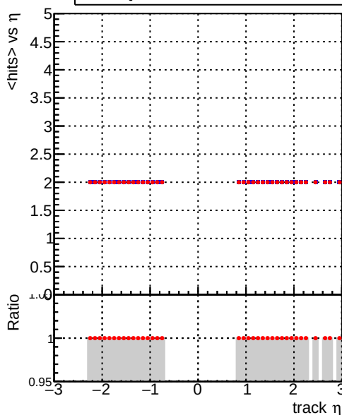
mean hits DQM_V0001_R000000001_Global_mkFit1000i0_RECO DQM_V0001_R000000001_Global_mkFit1000mod_RECO
