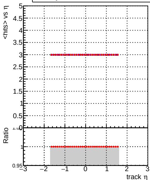
mean hit DQM_V0001_R000000001_Global_mkFit1000i0_RECO DQM_V0001_R000000001_Global_mkFit1000mod_RECO
