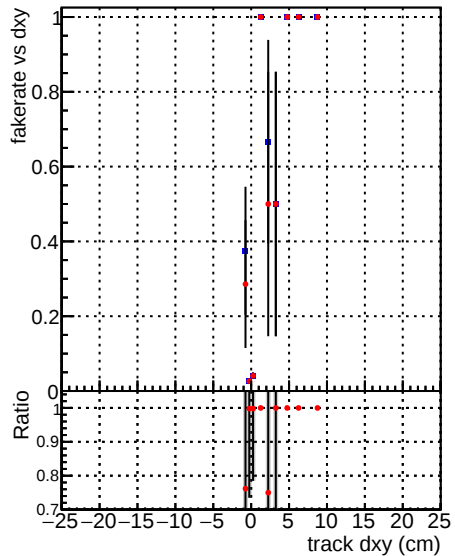
█ █ DQM V0001_R0000000001_Global_mkFiti100i0_RECO █ █ DQM V0001_R0000000001_Global_mkFiti1000mod_RECO
