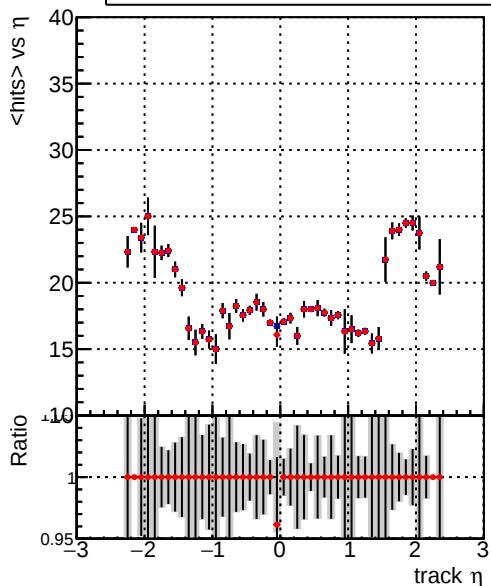
mean hits vs \eta — DQM_V0001_R000000001_Global_mkFit100i0_RECO — DQM_V0001_R000000001_Global_mkFit1000mod_RECO
