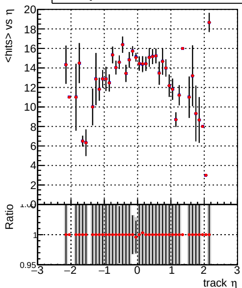
— DQM_V0001_R0000000001_Global_mkFit1000i0_RECO — DQM_V0001_R0000000001_Global_mkFit1000mod_RECO
