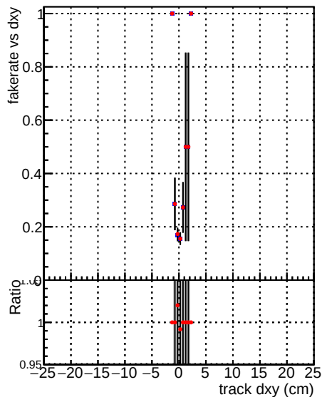
—●— DQM V0001_R000000001 Global mkFit1000i0_RECO —●— DQM V0001_R000000001 Global mkFit1000mod_RECO
