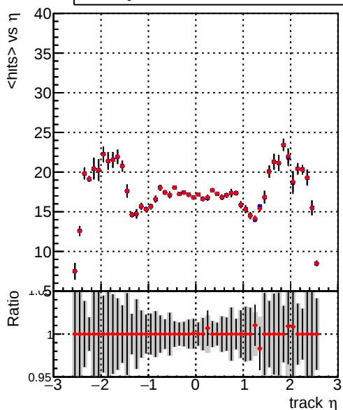
— DQM_V0001_R000000001_Global_mkFiti100i0_RECO — DQM_V0001_R000000001_Global_mkFiti1000mod_RECO
