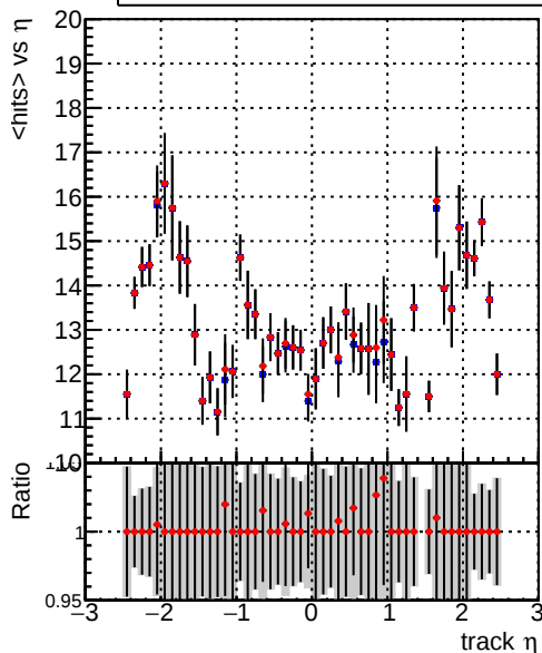
mean hit — DQM_V0001_R000000001_Global_mkFiti100i0_RECO — DQM_V0001_R000000001_Global_mkFiti1000mod_RECO
