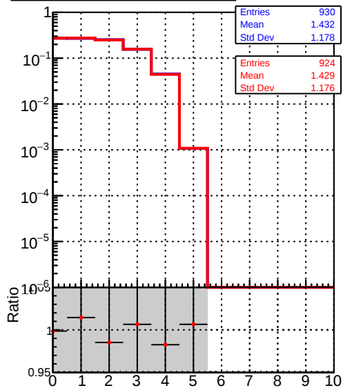
mean hit — DQM_V0001_R000000001_Global_mkFiti100i0_RECO — DQM_V0001_R000000001_Global_mkFiti1000mod_RECO
