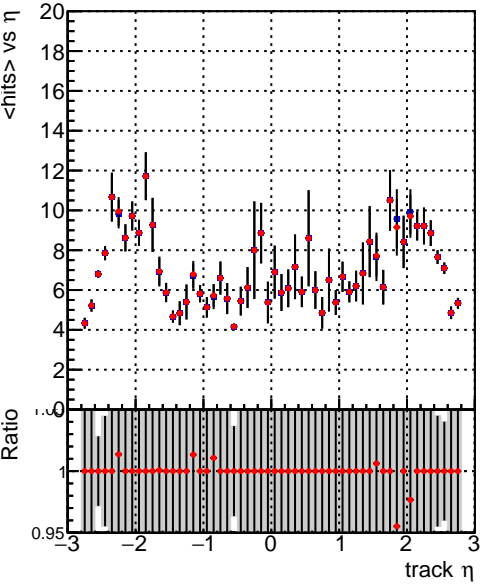
— DQM_V0001_R000000001_Global_mkFit100i0_RECO — DQM_V0001_R000000001_Global_mkFit1000mod_RECO
