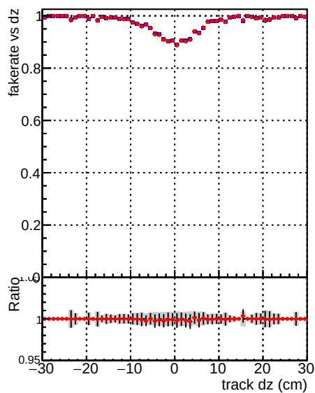
DQM_V0001_R000000001_Global_mkFiti100i0_RECO Fake rate vs d DQM_V0001_R000000001_Global_mkFiti100mod_RECO
