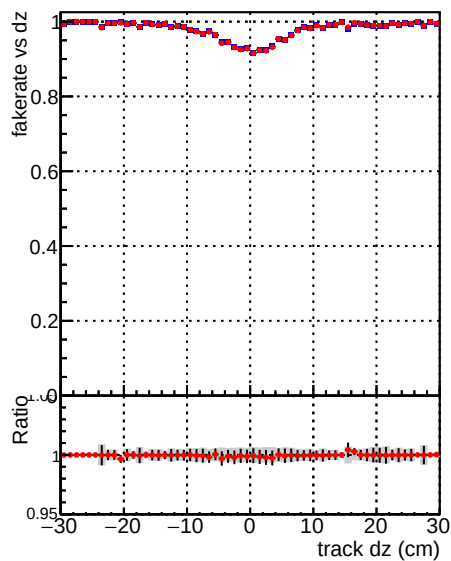
—●— DQM_V0001_R0000000001_Global_mkFiti100i0_RECO —●— DQM_V0001_R0000000001_Global_mkFiti1000mod_RECO
