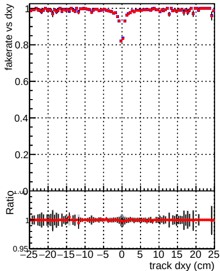
—●— DQM_V0001_R0000000001_Global_mkFiti100i0_RECO —●— DQM_V0001_R0000000001_Global_mkFiti1000mod_RECO
