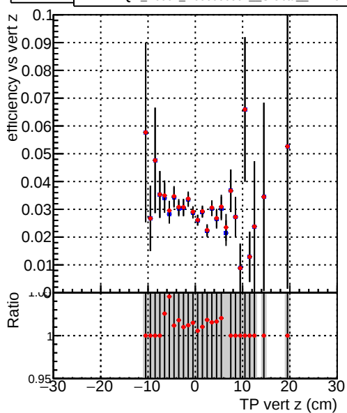
Efficiency vs. sim PV z — DQM_V0001_R000000001_Global_mkFit1000i0_RECO — DQM_V0001_R000000001_Global_mkFit1000mod_RECO
