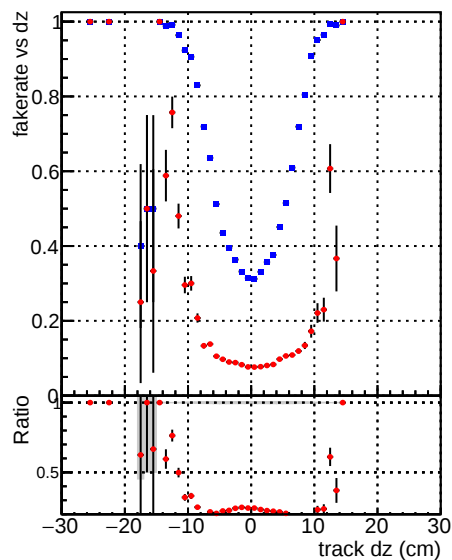
Fake rate vs dz DQM V0001_R000000001 Global mkFit1000i0_RECO DQM V0001_R000000001 Global mkFit1000mod_RECO
