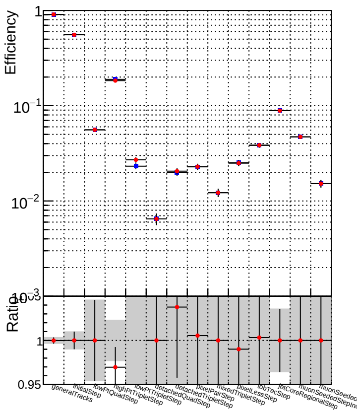
DQM_V0001_R000000001_Global_mkFiti100i0_RECO DQM_V0001_R000000001_Global_mkFiti1000mod_RECO
