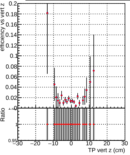
Efficiency vs TP vert z Legend: DQM_V0001_R000000001_Global_mkFiti100i0_RECO DQM_V0001_R000000001_Global_mkFiti1000mod_RECO
