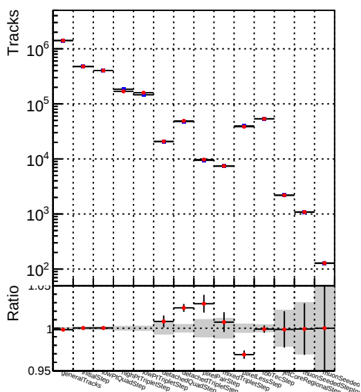
■ DQM_V0001_R0000000001_Global_mkFiti100i0_RECO
