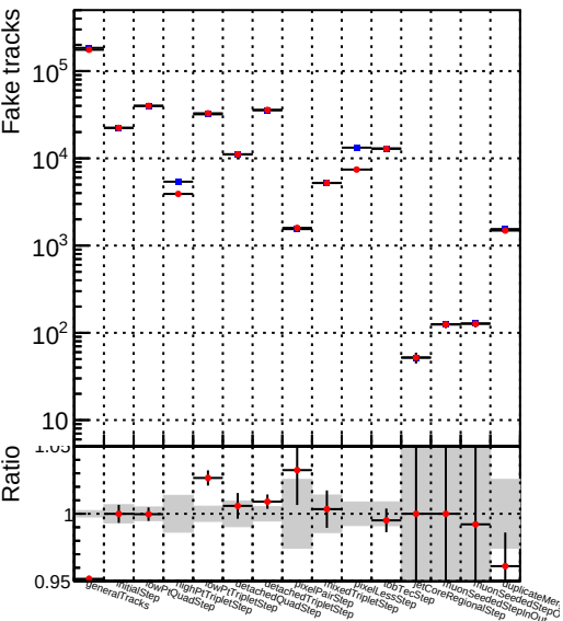
Number —●— DQM_V0001_R000000001_Global_mkFiti1000mod_RECO
