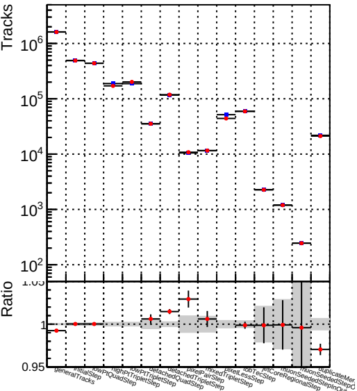
DQM_V0001_R000000001__Global__mkFiti100i0__RECO
