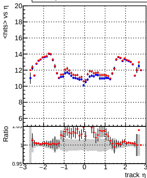
DQM_V0001_R000000001_Global_mkFit100i0_RECO mean hits DQM_V0001_R000000001_Global_mkFit1000mod_RECO
