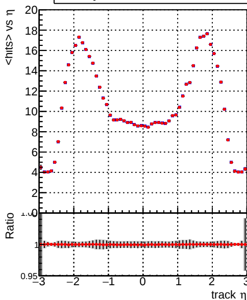
— DQM_V0001_R000000001_Global_mkFit100i0_RECO — DQM_V0001_R000000001_Global_mkFit1000mod_RECO
