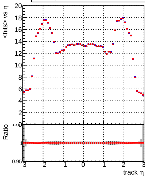
— DQM_V0001_R000000001_Global_mkFit100i0_RECO — DQM_V0001_R000000001_Global_mkFit1000mod_RECO
