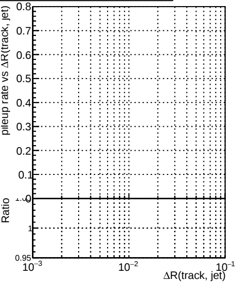
Legend: DQM_V0001_R000000001_Global_mkFiti100i0_RECO (blue squares), DQM_V0001_R000000001_Global_mkFiti1000mod_RECO (red circles)
