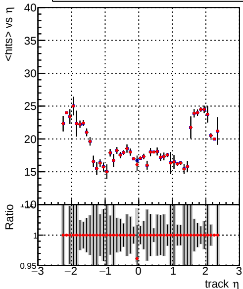
— DQM_V0001_R000000001_Global_mkFit100i0_RECO — DQM_V0001_R000000001_Global_mkFit1000mod_RECO
