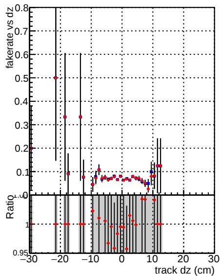
—●— DQM V0001_R0000000001_Global_mkFiti100i0_RECO —●— DQM V0001_R0000000001_Global_mkFiti1000mod_RECO
