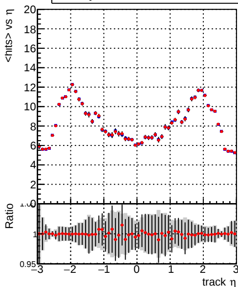
mean hits vs \eta Legend: DQM_V0001_R000000001_Global_mkFit100i0_RECO (blue line), DQM_V0001_R000000001_Global_mkFit1000mod_RECO (red line)
