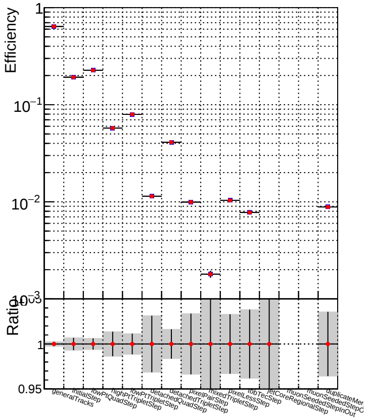
DQM_V0001_R0000000001_Global_mkFiti100i0_RECO DQM_V0001_R0000000001_Global_mkFiti1000mod_RECO
