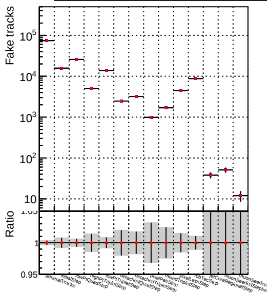
Number ● DQM_V0001_R000000001_Global_mkFiti1000mod_RECO
