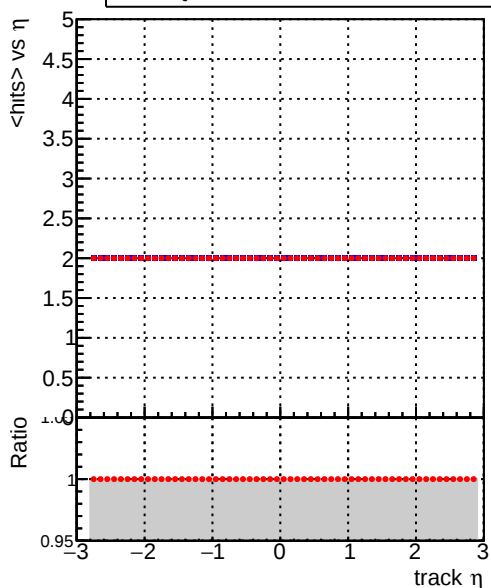
mean hits vs \eta Legend: DQM_V0001_R000000001_Global_mkFit1000i0_RECO (blue line), DQM_V0001_R000000001_Global_mkFit1000mod_RECO (red line)
