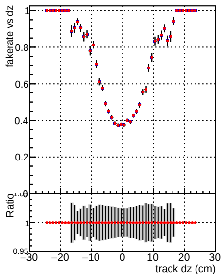
Fake rate vs d Legend Series Blue line with square markers DQM_V0001_R0000000001_Global_mkrFiti1000b_RECO Red line with circle markers DQM_V0001_R0000000001_Global_mkFiti1000mod_RECO
