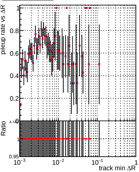
Legend: \blacksquare DQM_V0001_R000000001_Global_mkFiti100i0_RECO \bullet DQM_V0001_R000000001_Global_mkFiti1000mod_RECO
