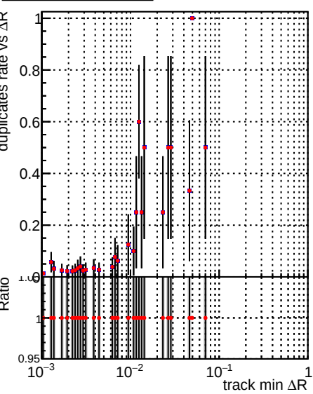
Legend: \blacksquare DQM_V0001_R000000001_Global_mkFiti100i0_RECO \bullet DQM_V0001_R000000001_Global_mkFiti1000mod_RECO
