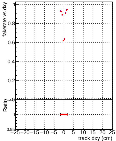
Fake rate vs d DQM_V0001_R0000000001_Global_mkFit1000i0_RECO DQM_V0001_R0000000001_Global_mkFit1000mod_RECO
