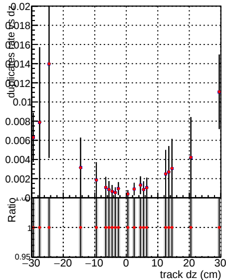
—●— DQM_V0001_R0000000001 Global mkFit100i0 RECO —●— DQM_V0001_R0000000001 Global mkFit1000mod RECO
