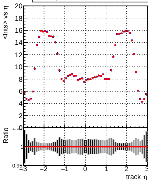
— DQM_V0001_R000000001_Global_mkFiti100i0_RECO — DQM_V0001_R000000001_Global_mkFiti1000mod_RECO
