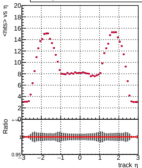
— DQM_V0001_R000000001_Global_mkFit100i0_RECO — DQM_V0001_R000000001_Global_mkFit1000mod_RECO
