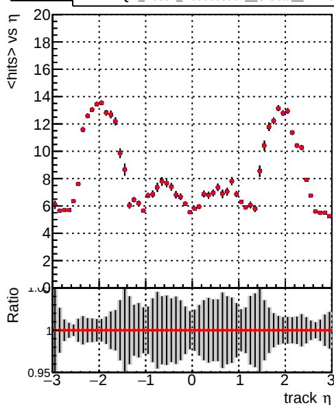
— DQM_V0001_R0000000001_Global_mkFit100i0_RECO — DQM_V0001_R0000000001_Global_mkFit1000mod_RECO
