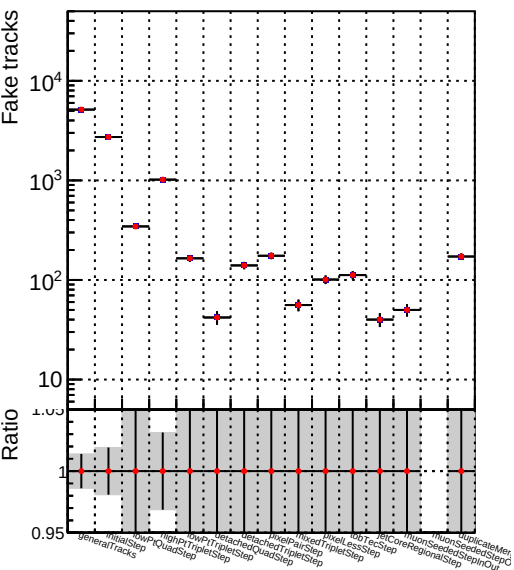
Number —●— DQM_V0001_R000000001_Global_mkFiti1000mod_RECO
